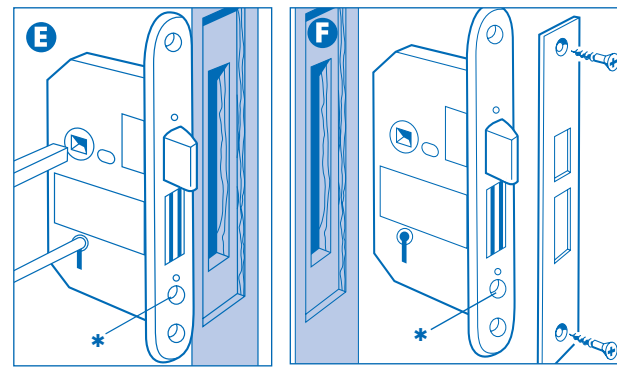
Mark and drill holes
