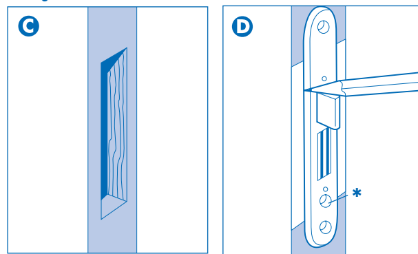
Chisel out mortice
