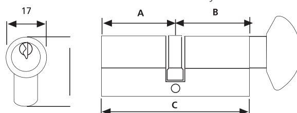
BS Double Euro Profile Thumbturn Cylinder
